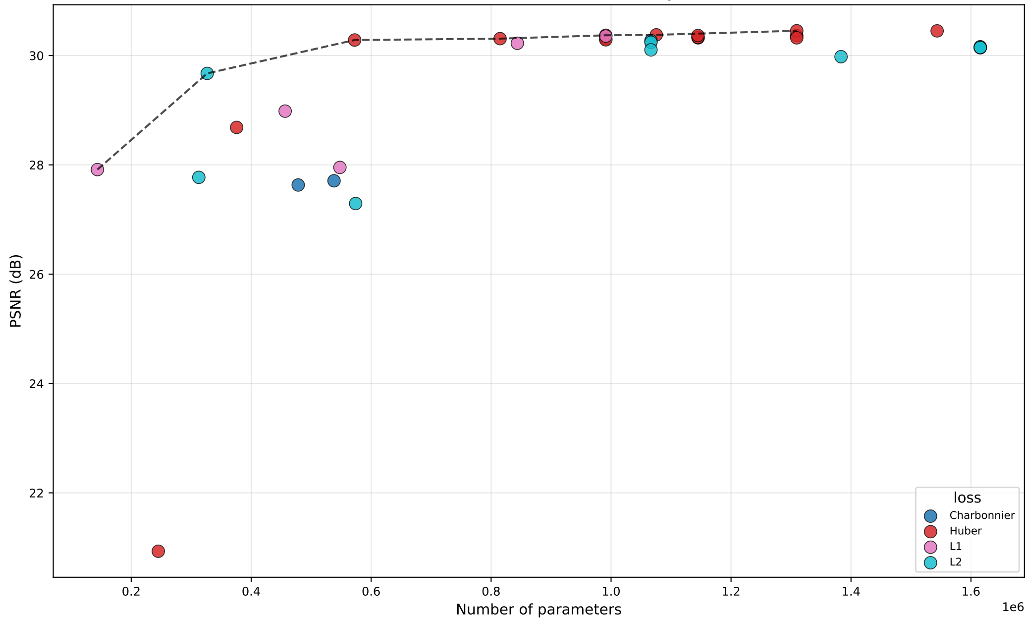
PSNR vs #Params — SRFormer — by loss
